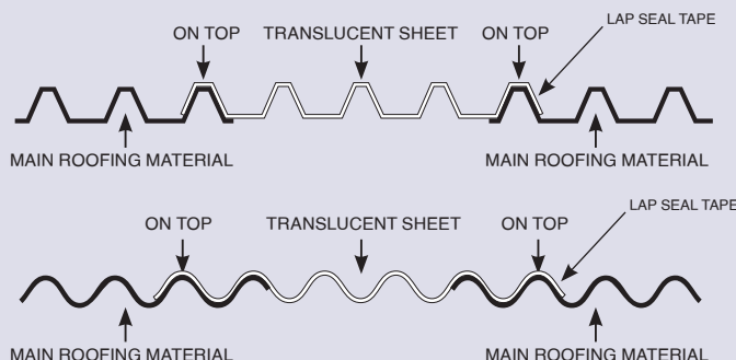
Figure 1 - Laserlite Building Products recommends the use of a strip of 24mm x 5mm Lap Seal Tape
